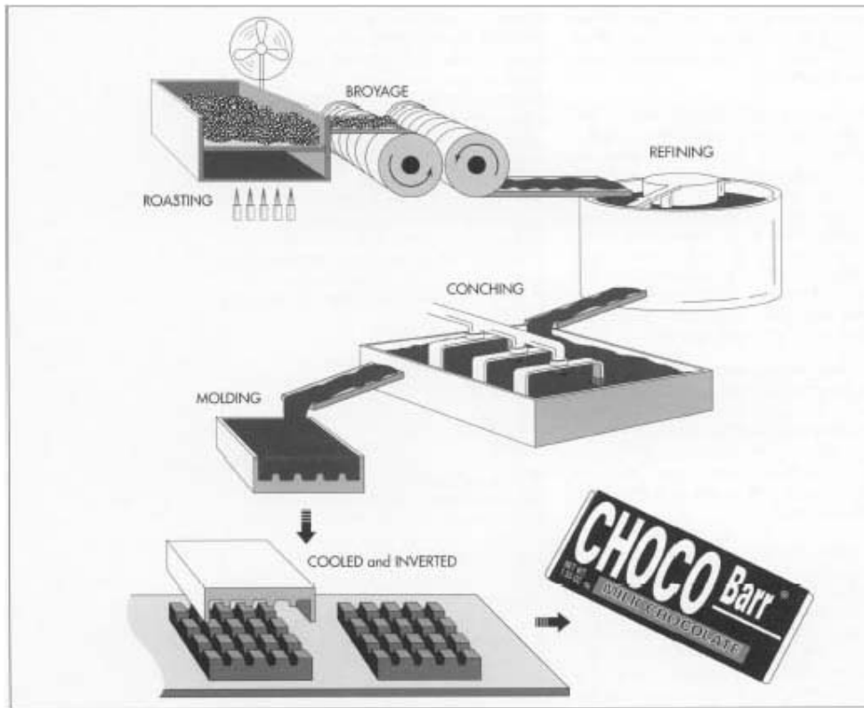
Figure 1 Schematic process of chocolate
